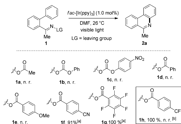
Scheme 3. Screening of acyl oxime substrates. Reaction conditions: A mixture of 1 (0.1 mmol) and fac-[Ir(ppy)_3] (0.001 mmol, 1.0 mol%) in dry DMF (2.0 mL) was irradiated by 5 W white light-emitting diodes (LEDs) for 10 h. Yields were determined by ^1\text{H} NMR spectroscopic analysis. [a] The reaction time was prolonged to 24 h. [b] Result observed (no reaction) without a photocatalyst or irradiation with visible light. n. r. = no reaction. DMF = N,N -dimethylformamide.
