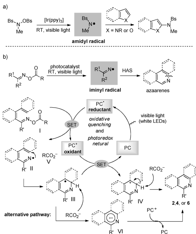
Scheme 2. Rationale for the synthesis of six-membered azaarenes. a) Previously reported visible-light-promoted C–H amination via amidyl radicals (Bs = benzenesulfonyl). b) Visible-light-promoted synthesis of azarenes via iminyl radicals (present study).
