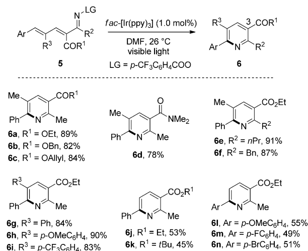
Scheme 6. Scope of the transformation of acyl oximes into pyridines. Reaction conditions: A mixture of 5 (0.2 mmol) and fac\text{-}[\text{Ir}(\text{ppy})_3] (0.002 mmol, 1.0 mol%) in dry DMF (4.0 mL) was irradiated by 5 W white LEDs for 10 h. Yields are for the isolated product.
